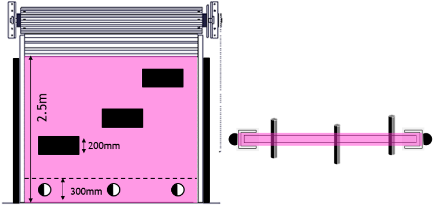
Test piece A is oriented with the 200mm dimension vertical.
