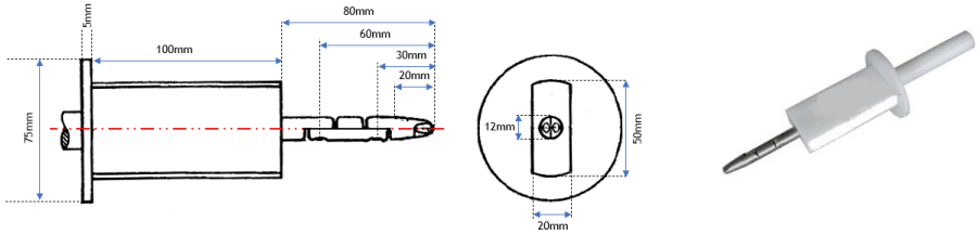
Test probe B according to EN 61032
