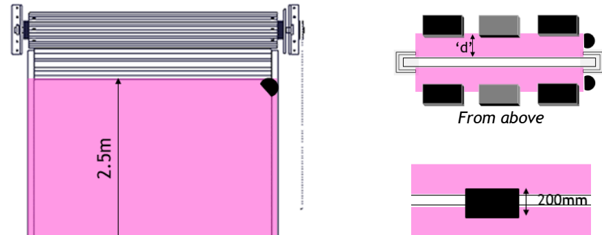
Placed on the floor with the 200mm dimension horizontal to test the dead zone
