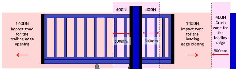
Examples of maximum force at differing hazard locations
