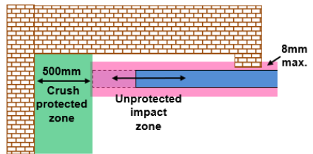
Sliding door/gate
