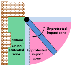
Swing door/gate
